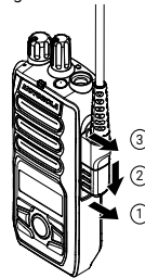
Figure 2: Remove the accessory connector
