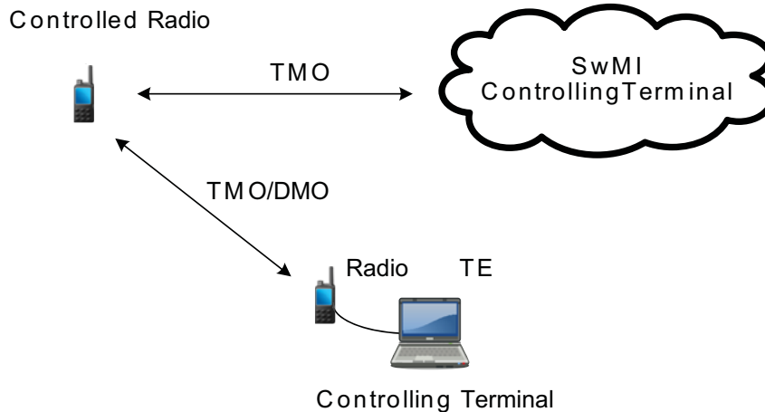
Figure 8: SDS Remote Control Overview
