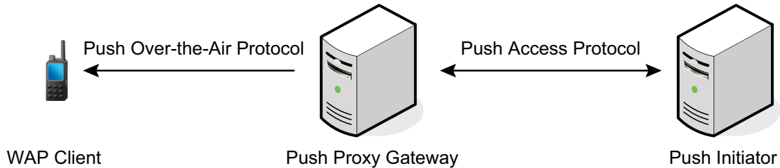
Figure 9: Push Framework
