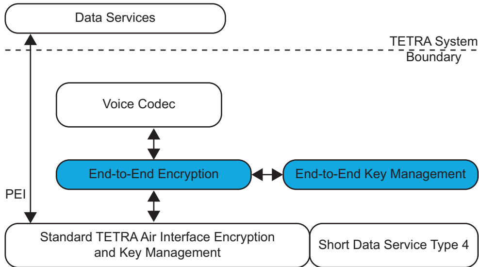
Figure 12: Voice and Data End to End Encryption
