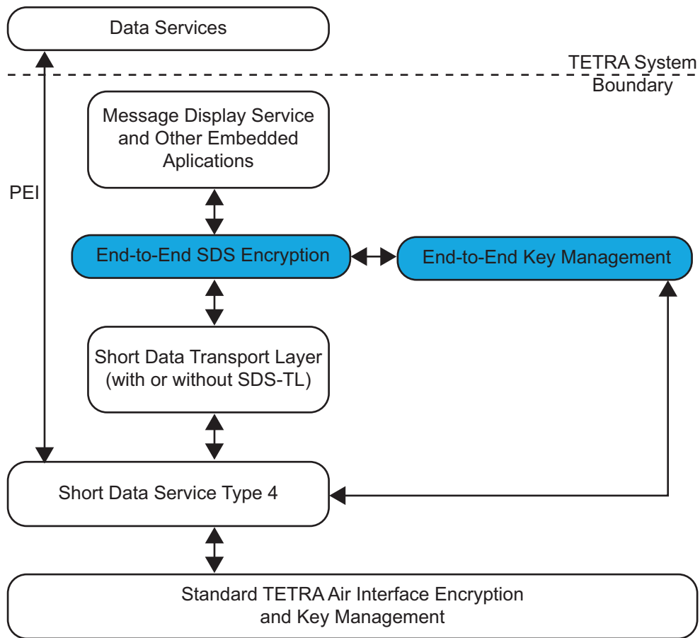
Figure 11: SDS End-to-End Encryption
