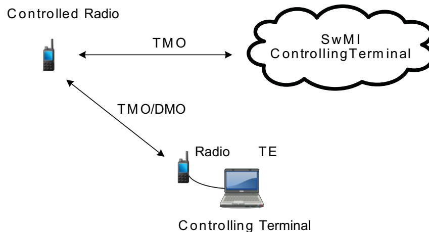
Figure 13: SDS Remote Control Overview
