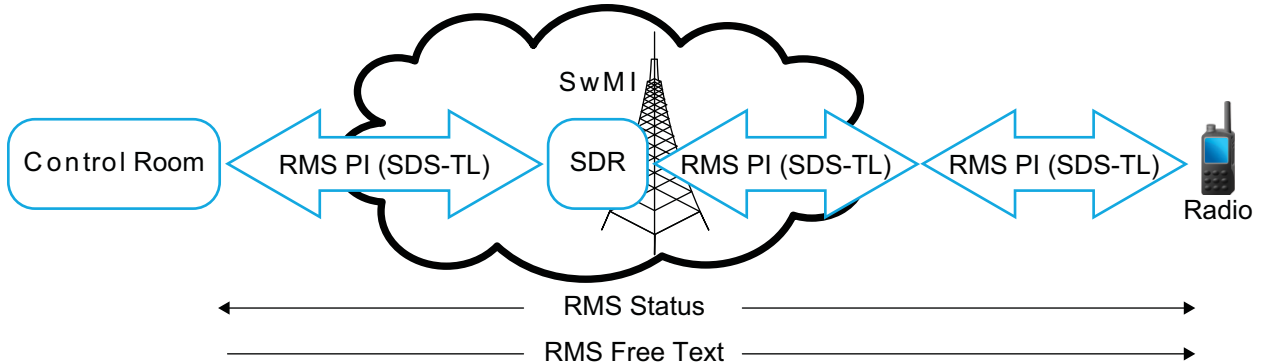
Figure 14: RMS Flow Model with SDS TL
