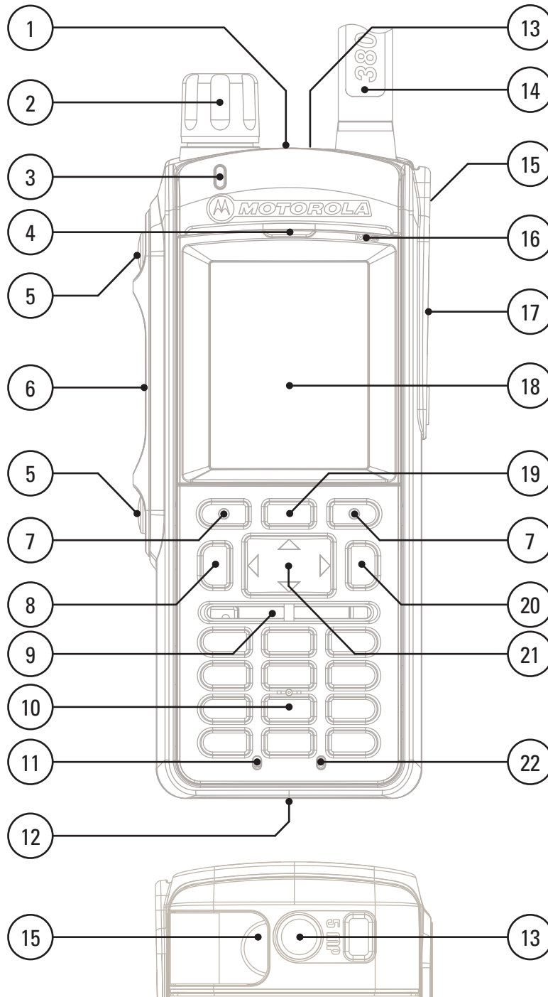
Figure 18: MTP6000 Series Controls and Indicators
