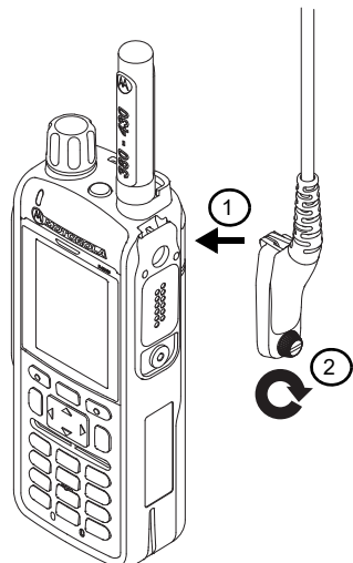
Figure 1: Securing the accessory connector
