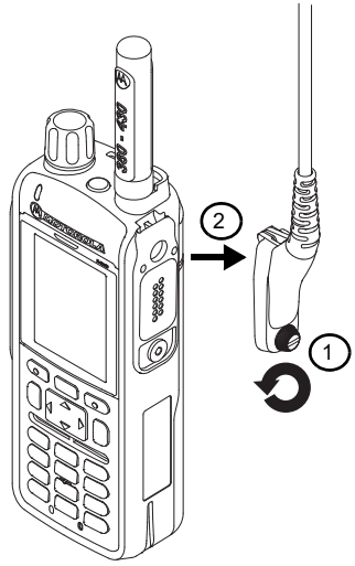
Figure 2: Removing the accessory connector
