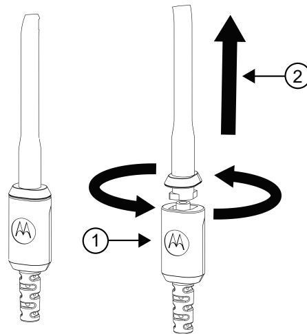
Figure 6: Translucent Acoustic Tube Replacement
