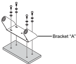
Figure 1: Installing Bracket "A"
