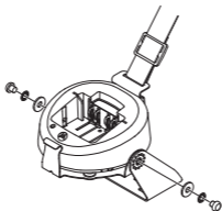
Figure 5: Mounting VCM-5 Bracket to Bracket "A"
