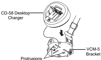
Figure 3: Inserting CD-58 Desktop Charger into VCM-5 Bracket
