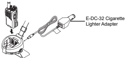
Figure 7: Connecting E-DC-32 Cigarette Lighter Adapter to CD-58 Desktop Charger
