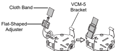
Figure 2: Installing Cloth Band and Flat-Shaped Adjuster
