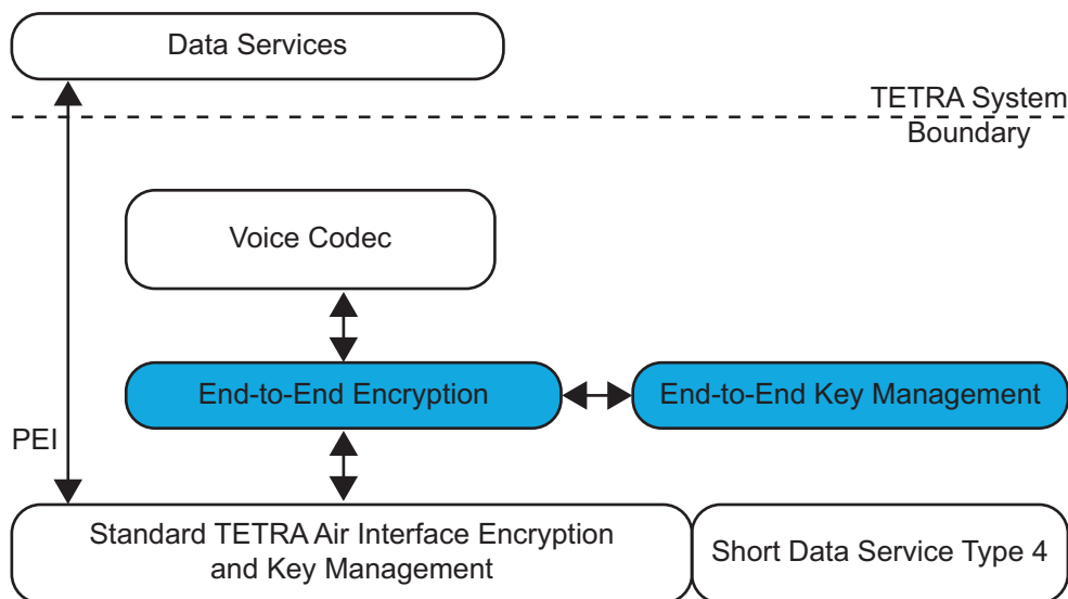
Figure 13: Voice and Data End to End Encryption
