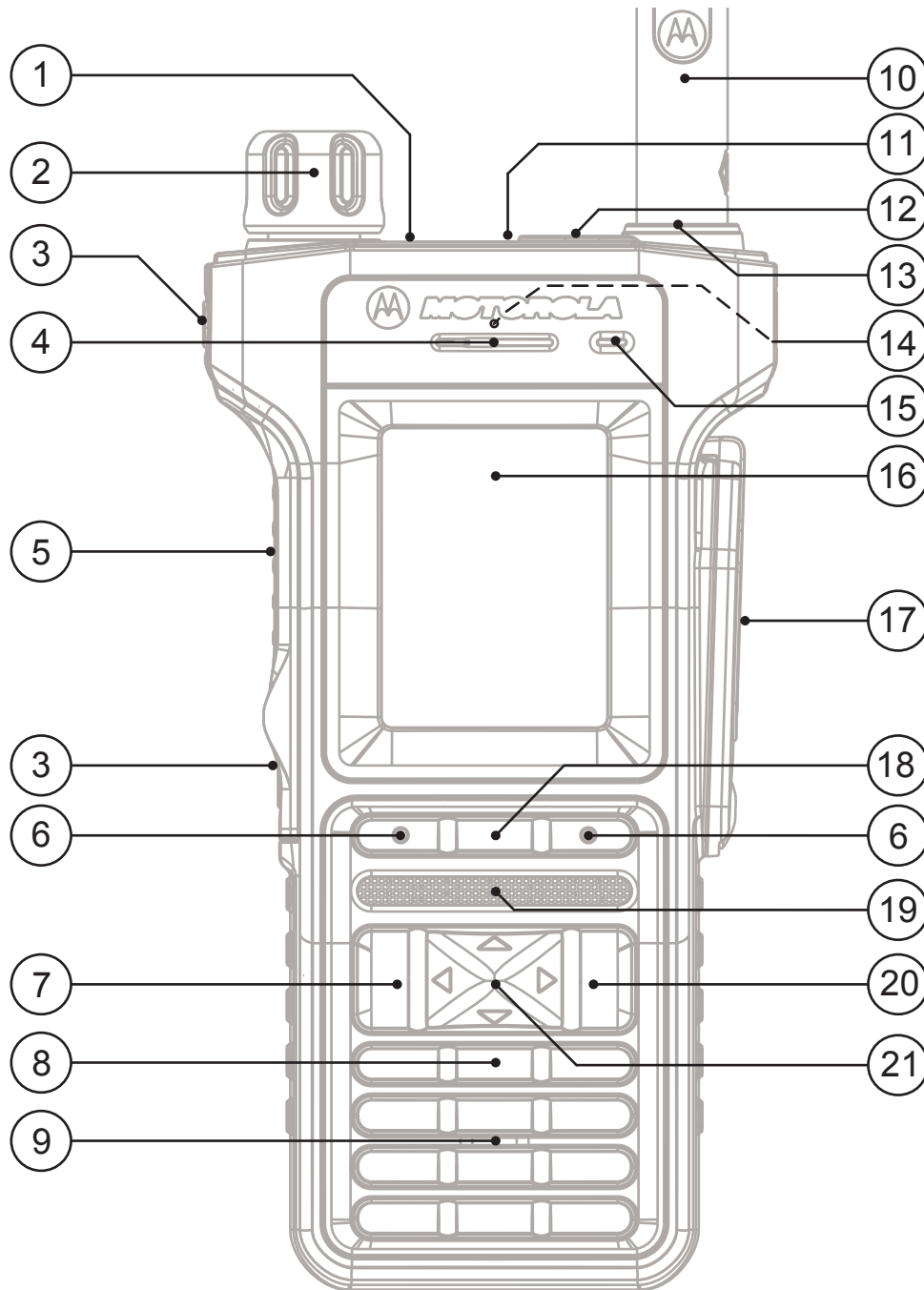
Figure 2: MTP8550Ex Controls and Indicators
