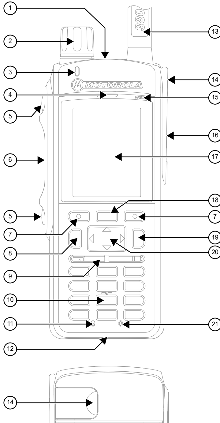
Figure 16: MTP6650 Controls and Indicators
