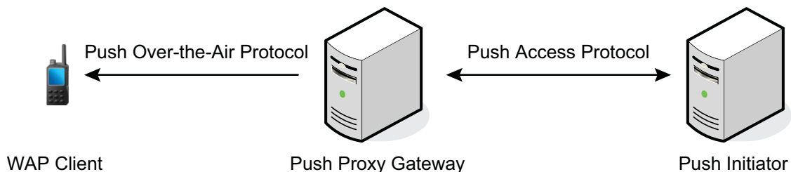
Figure 14: Push Framework
