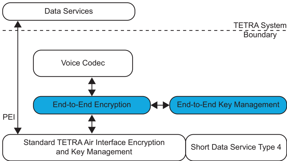
Figure 10: Voice and Data End to End Encryption
