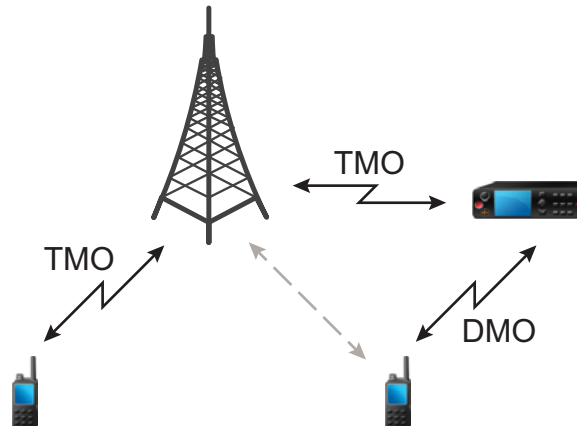
Figure 6: Communication Through Gateways
