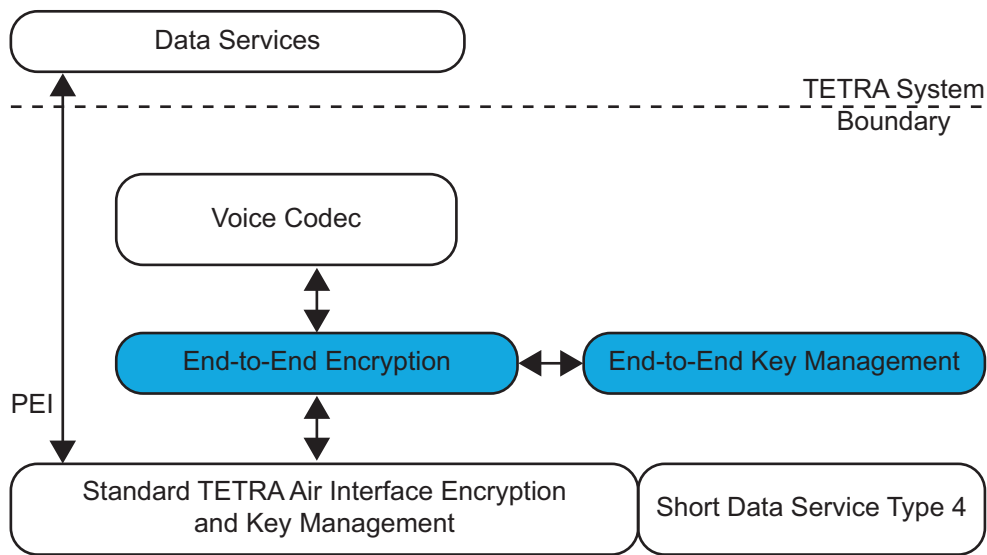
Figure 9: Voice and Data End to End Encryption
