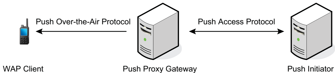
Figure 11: Push Framework
