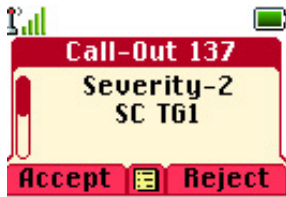
Figure 4: Call-Out Message
