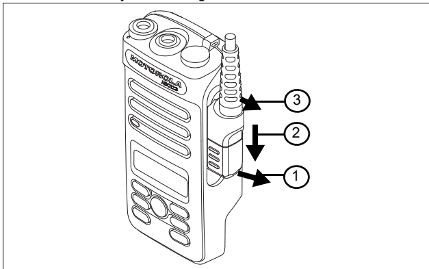
Figure 2: Remove the accessory connector
