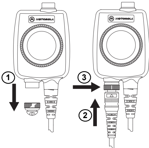
Figure 3. Attaching Remote PTT
