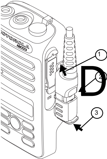
Figure 1: Secure the accessory connector
