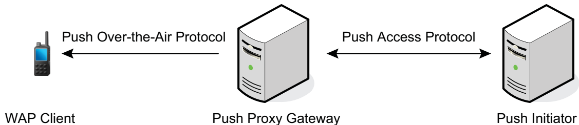
Figure 11: Push Framework
